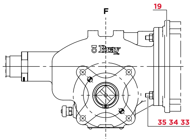
STANDARD Adapter
