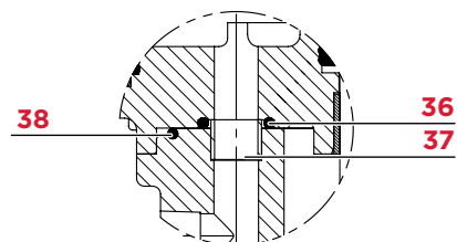
DETAIL C
