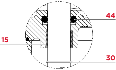
DETAIL C
