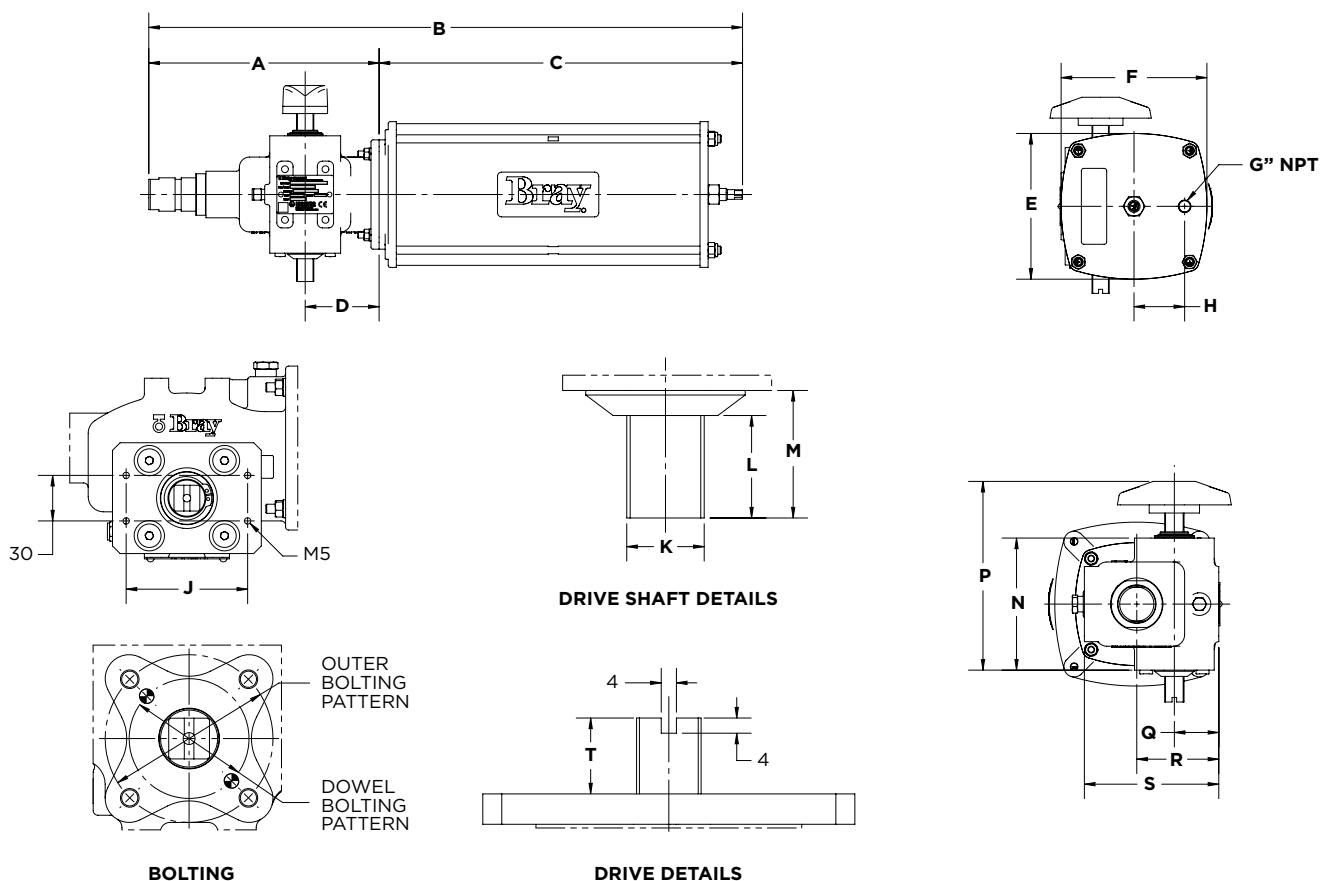
SERIES 98C MAX DIMENSIONS, mm
