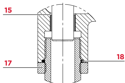
DETAIL E
