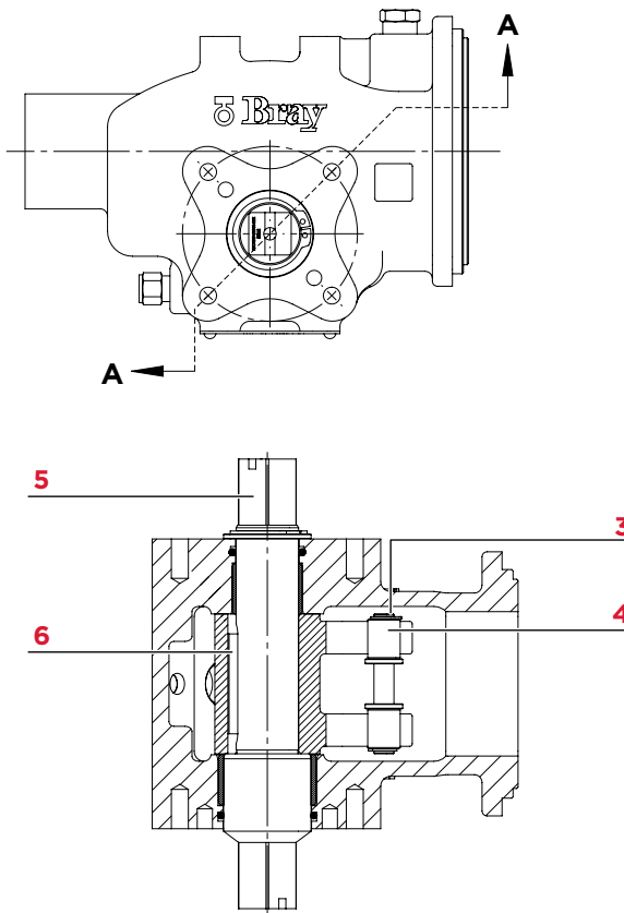
SECTION VIEW - A
