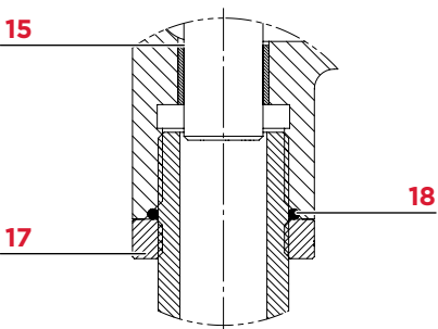
DETAIL E
