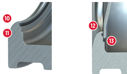
Figure 06: Integral Soft Seat Close-Up Cutaway Views.
